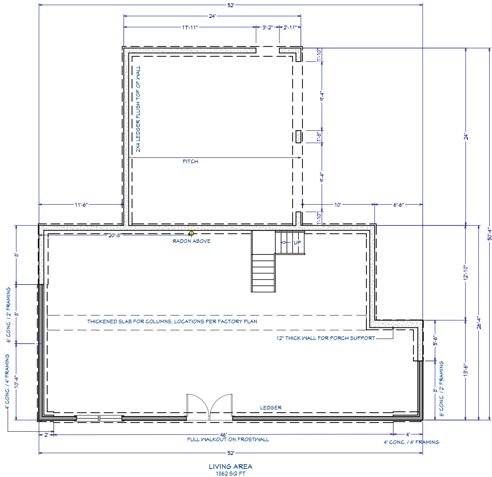
LOT 40 - FOUNDATION PLAN
